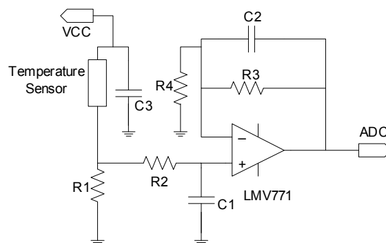
Figure 9: Schematic of the water pipe temperature sensor interface circuitry
