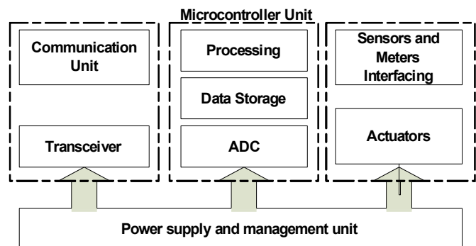
Figure 1: Top level system block diagram of the WSN mote
