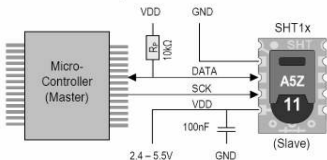
Figure 4: Typical application circuit of the SHT11
