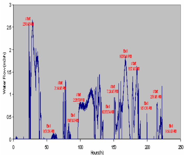
Figure 8: Water flow rate measurements
